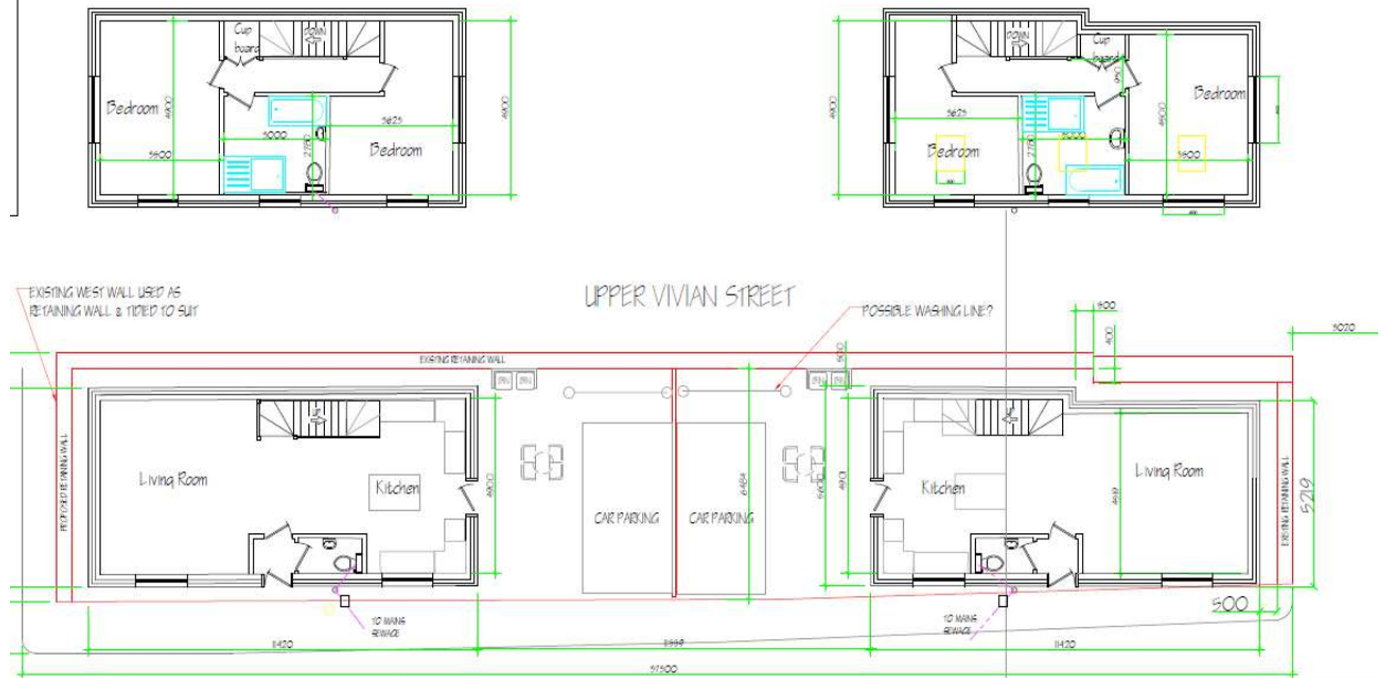
Figure 1.3 Proposed floor plans of each dwelling.
